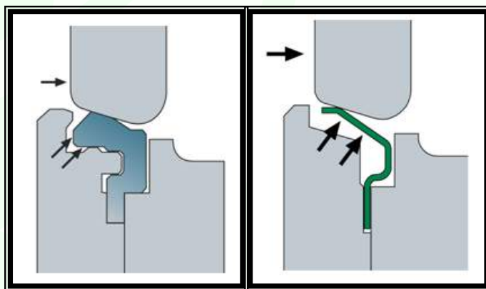
R-PTFE Seat
